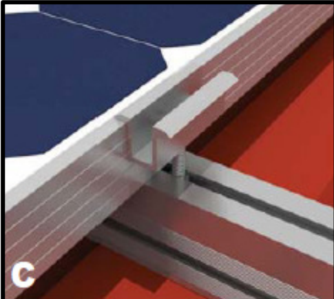
C Middle clamber
