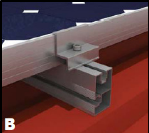
B Side clamber
